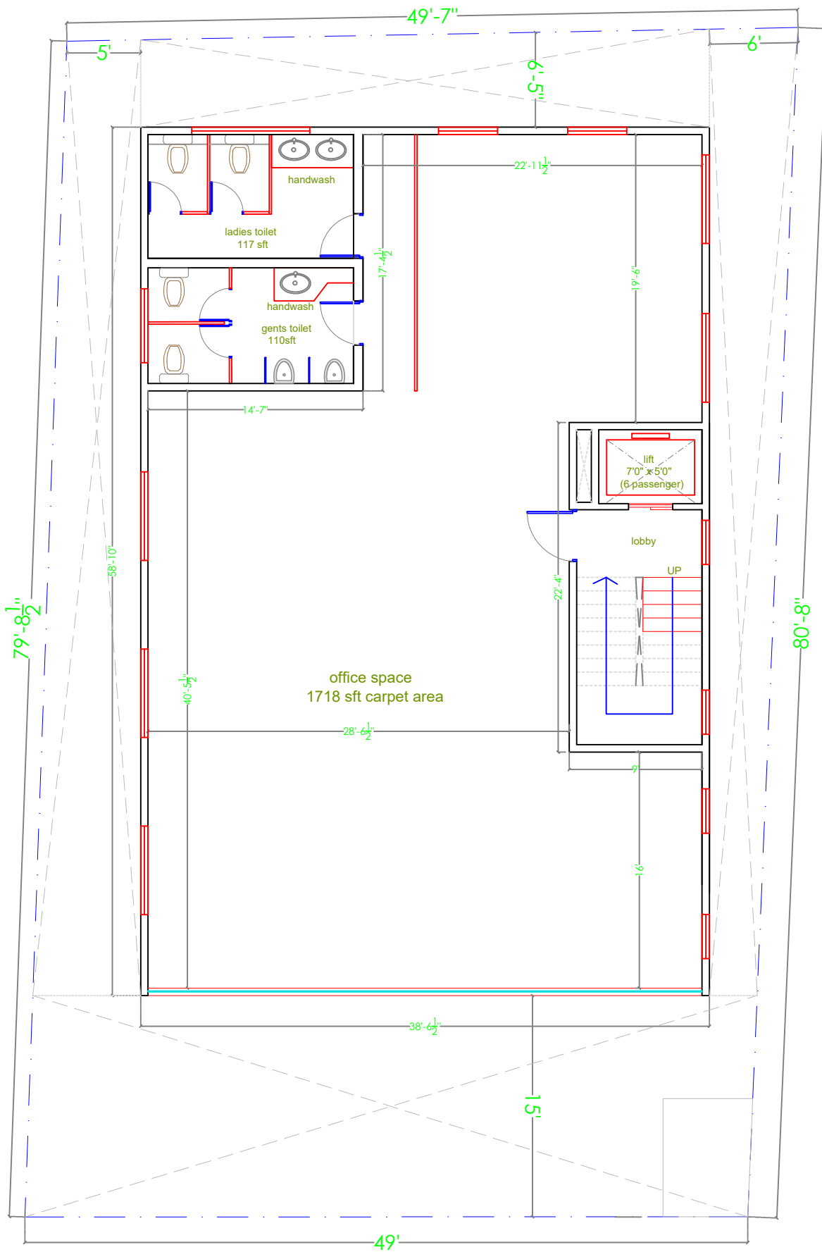
first, second floor plan (site area 3946.24) builtup : 2268sft (2nos)
